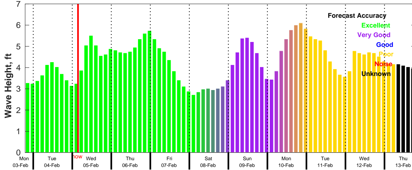
CMEMS Wave Forecast for NDBC 41013 from 03-Feb-2025 19:00:00 to 13-Feb-2025 19:00:00
