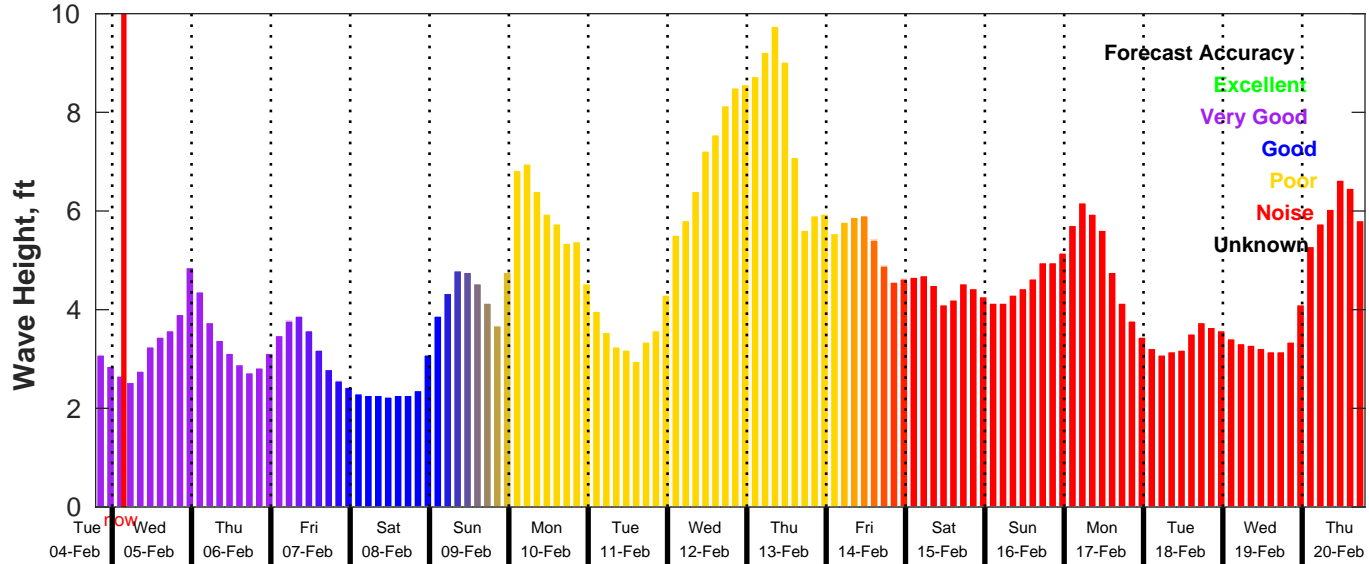
GFS Wave Forecast for NDBC 41013 from 04-Feb-2025 19:00:00 to 20-Feb-2025 19:00:00
