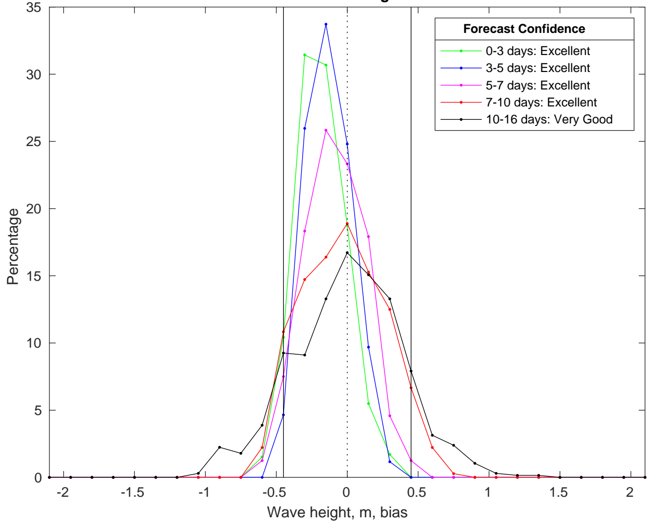
NDBC 41040 vs GFSWaves Bias Histogram: 05-Feb-2025
