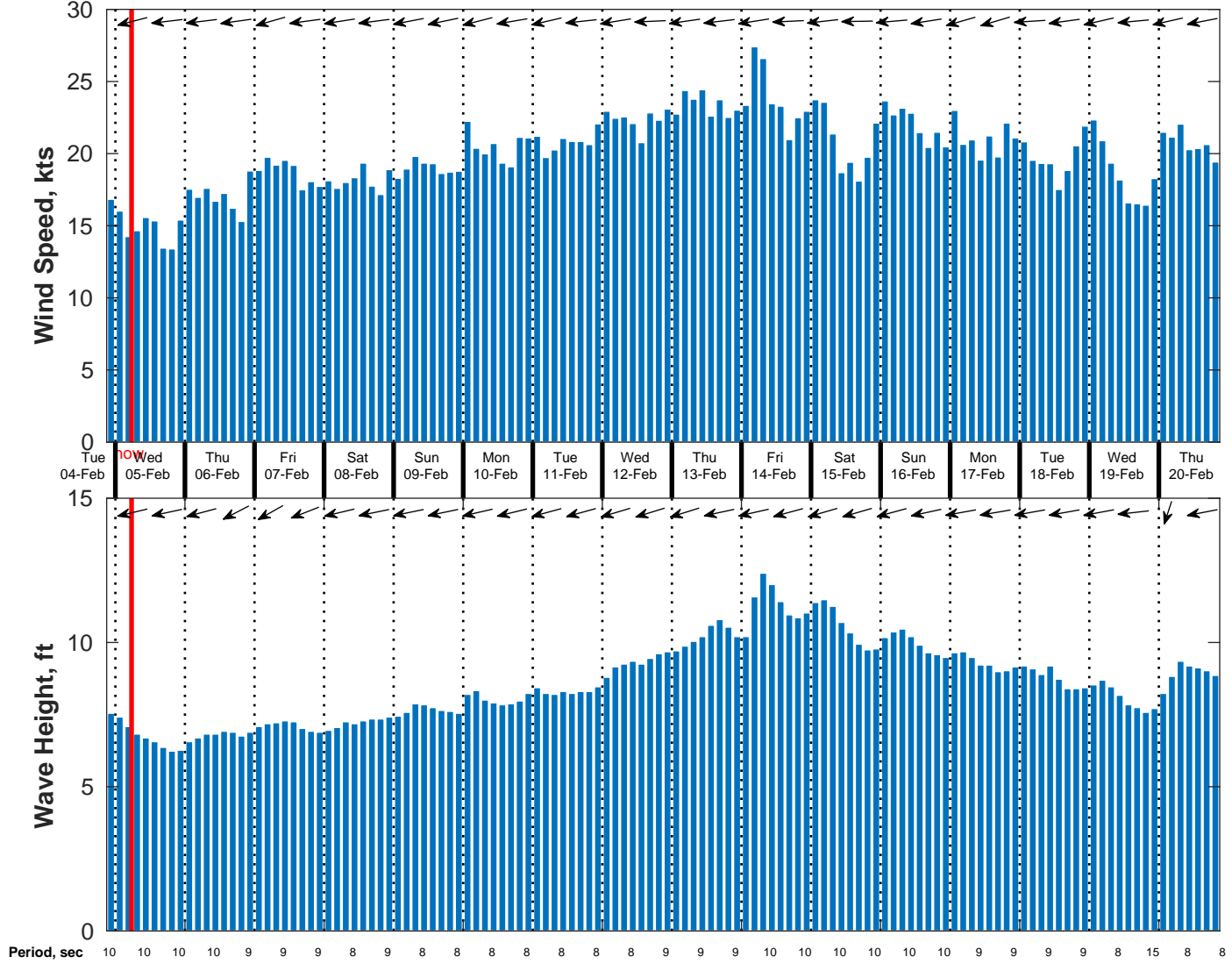
Wind & Wave Forecast for NDBC 41040 from 04-Feb-2025 21:00:00 to 20-Feb-2025 21:00:00
