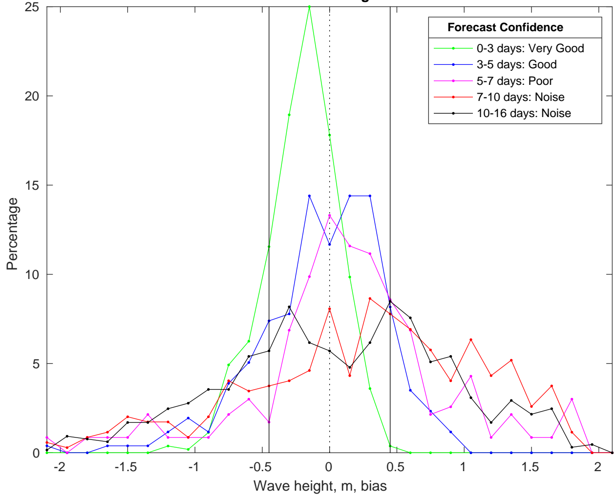
NDBC 42019 vs GFSWaves Bias Histogram: 05-Feb-2025
