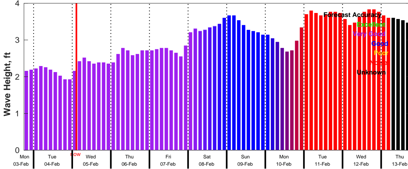
CMEMS Wave Forecast for NDBC 42019 from 03-Feb-2025 18:00:00 to 13-Feb-2025 18:00:00
