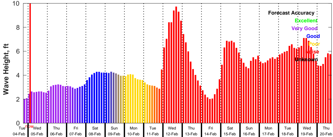
GFS Wave Forecast for NDBC 42019 from 04-Feb-2025 18:00:00 to 20-Feb-2025 18:00:00
