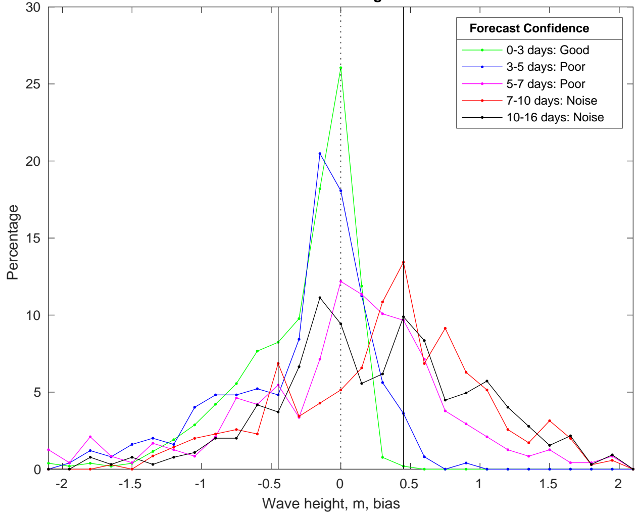
NDBC 42020 vs GFSWaves Bias Histogram: 05-Feb-2025
