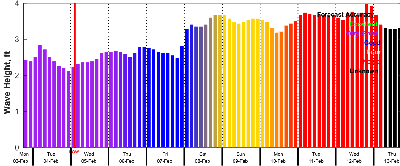
CMEMS Wave Forecast for NDBC 42020 from 03-Feb-2025 18:00:00 to 13-Feb-2025 18:00:00
