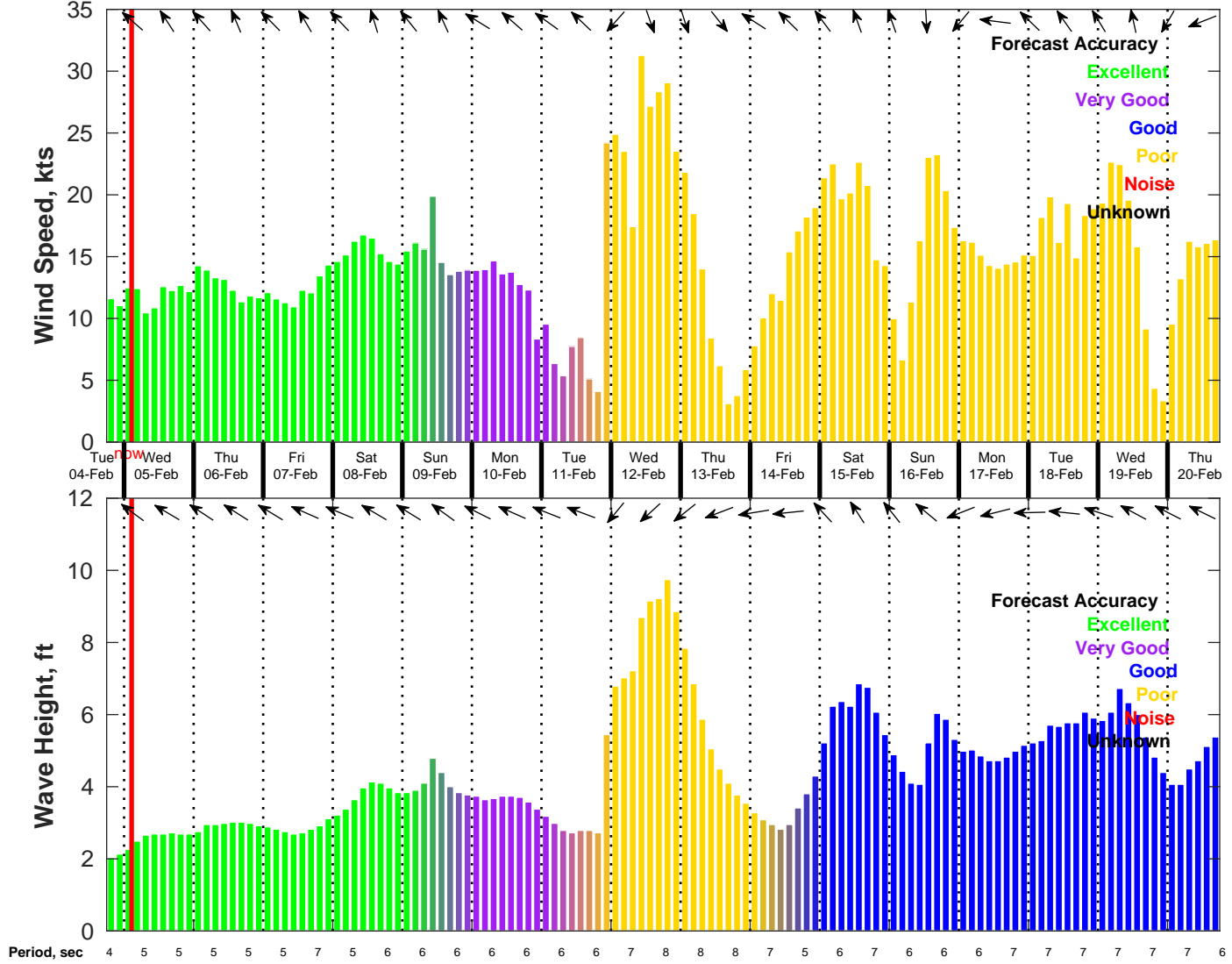
Wind & Wave Forecast for NDBC 42020 from 04-Feb-2025 18:00:00 to 20-Feb-2025 18:00:00
