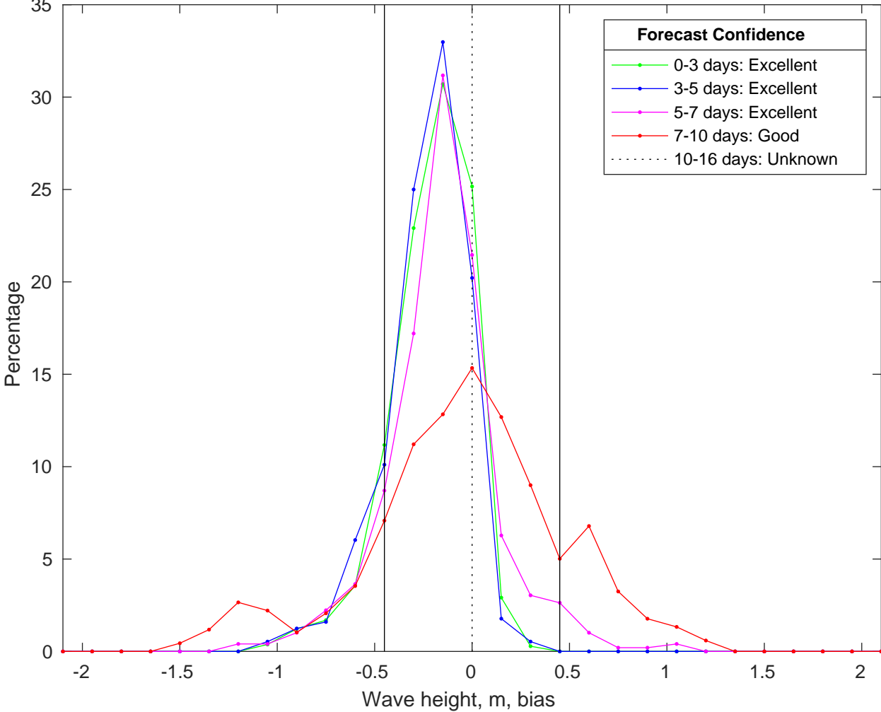
NDBC 42035 vs CMEMSWaves Bias Histogram: 05-Feb-2025
