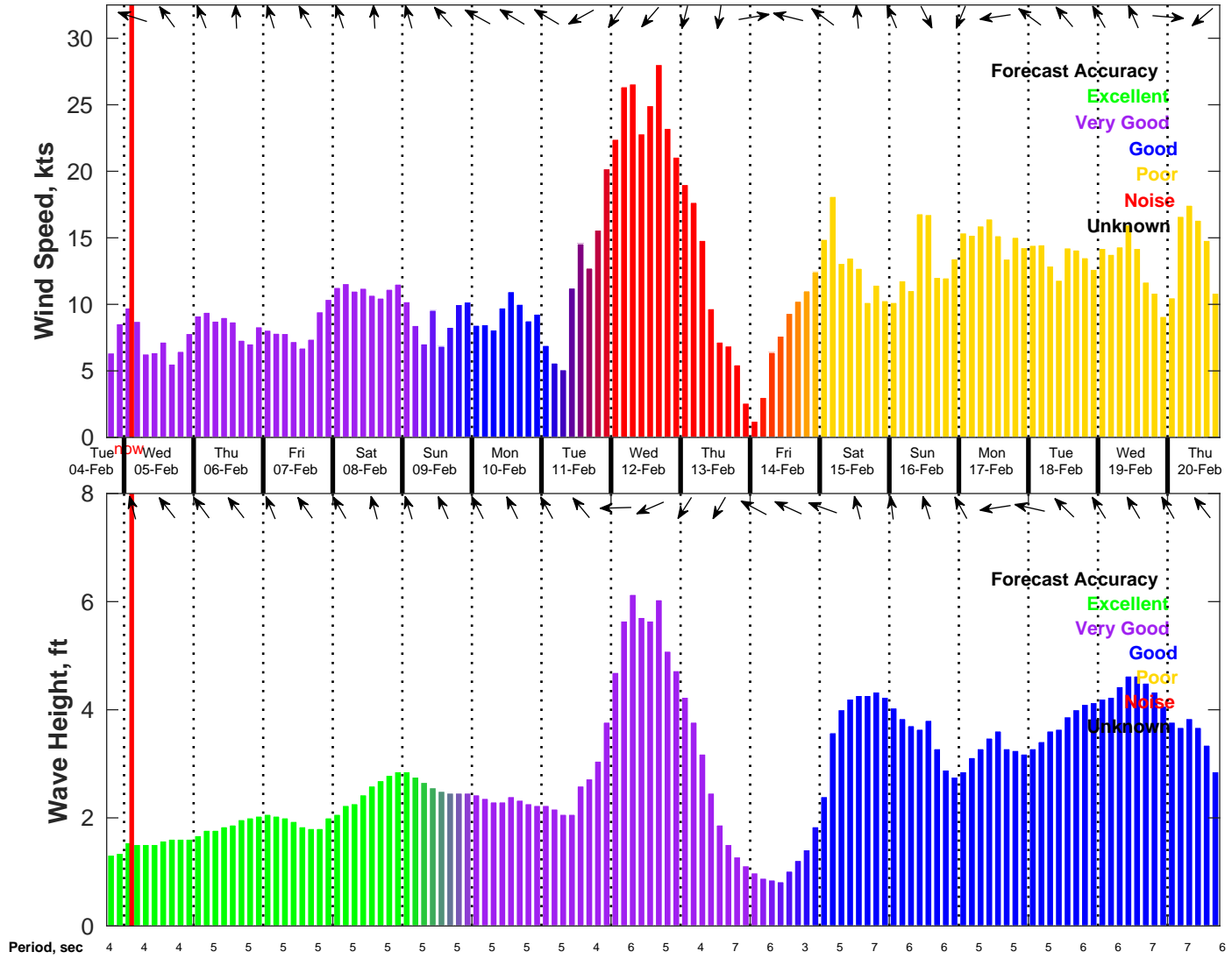
Wind & Wave Forecast for NDBC 42035 from 04-Feb-2025 18:00:00 to 20-Feb-2025 18:00:00
