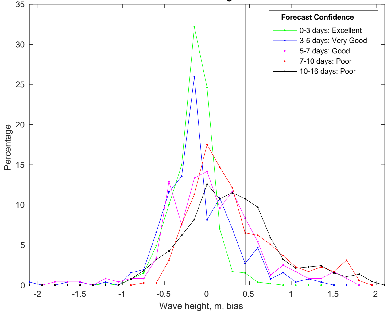
NDBC 42036 vs GFSWaves Bias Histogram: 05-Feb-2025
