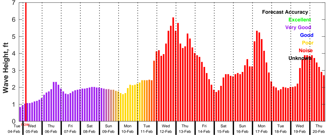
GFS Wave Forecast for NDBC 42040 from 04-Feb-2025 19:00:00 to 20-Feb-2025 19:00:00
