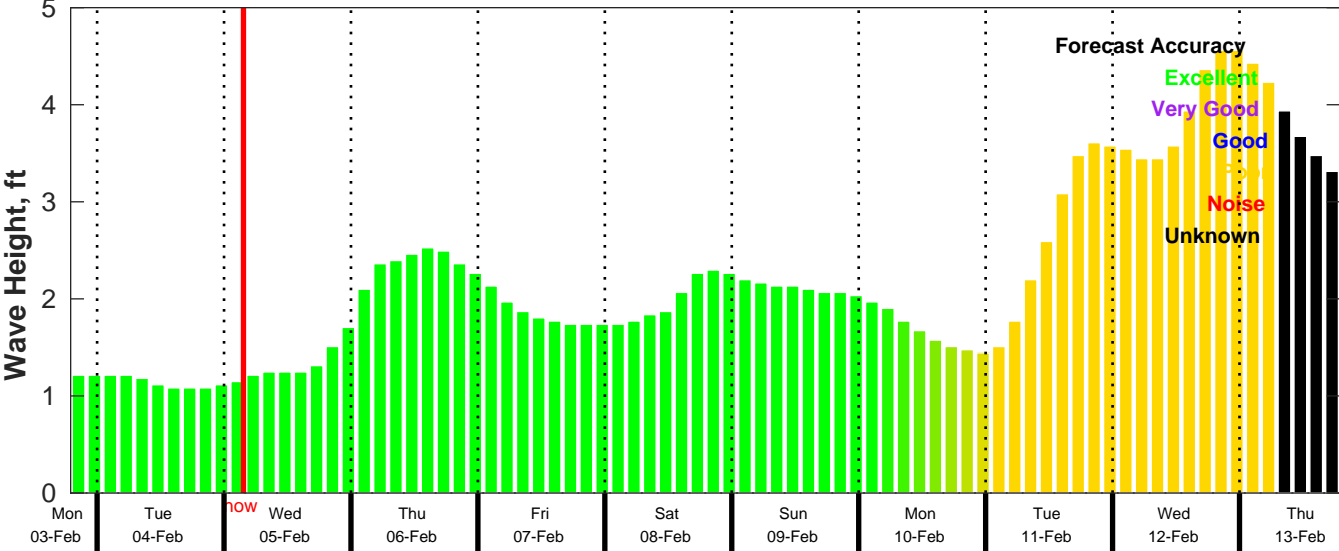
CMEMS Wave Forecast for NDBC 42084 from 03-Feb-2025 19:00:00 to 13-Feb-2025 19:00:00
