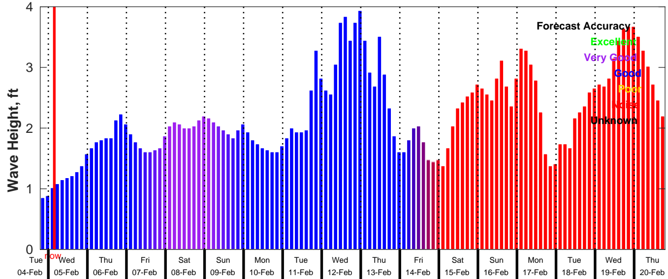
GFS Wave Forecast for NDBC 42084 from 04-Feb-2025 19:00:00 to 20-Feb-2025 19:00:00
