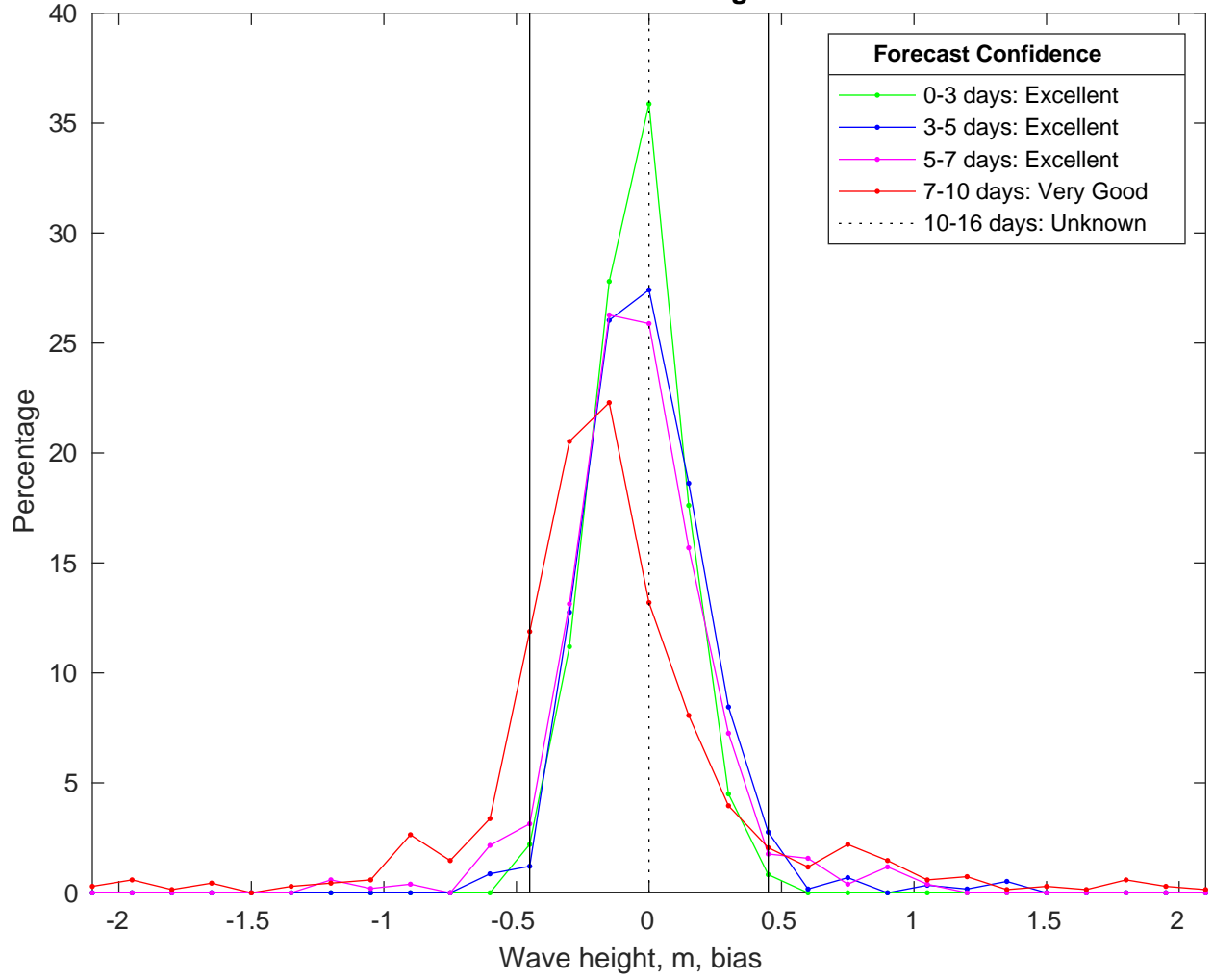
NDBC 46011 vs CMEMSWaves Bias Histogram: 05-Feb-2025
