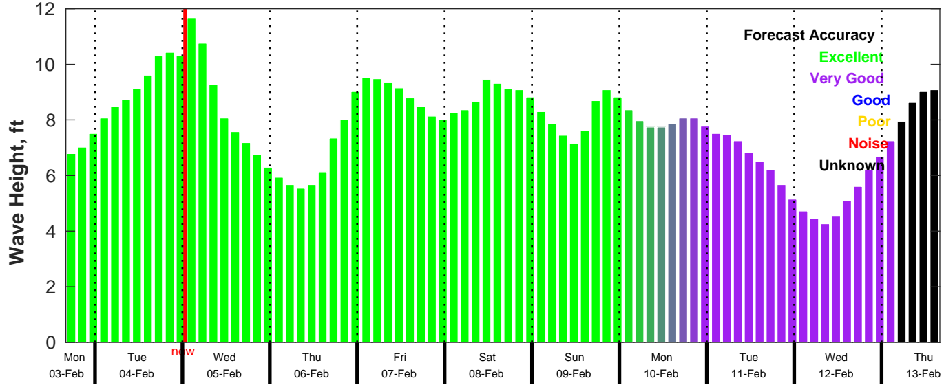
CMEMS Wave Forecast for NDBC 46028 from 03-Feb-2025 16:00:00 to 13-Feb-2025 16:00:00
