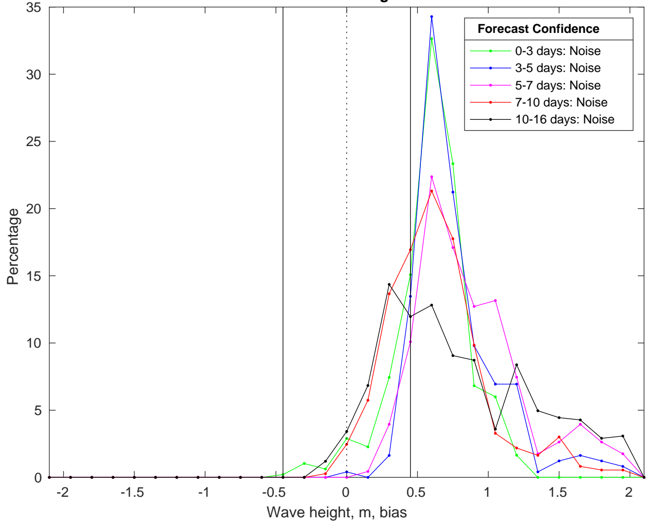
NDBC 46053 vs GFSWaves Bias Histogram: 03-Feb-2025
