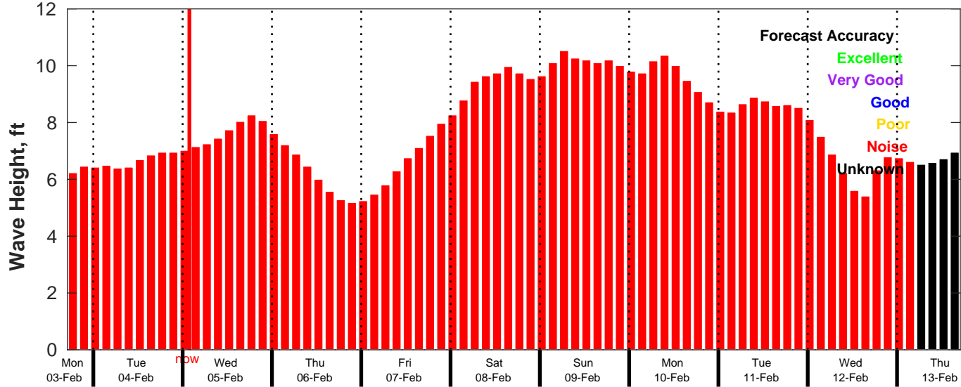
CMEMS Wave Forecast for NDBC 46053 from 03-Feb-2025 17:00:00 to 13-Feb-2025 17:00:00
