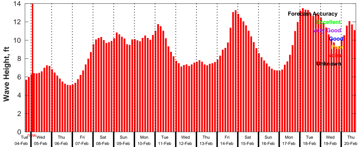
GFS Wave Forecast for NDBC 46053 from 04-Feb-2025 17:00:00 to 20-Feb-2025 17:00:00
