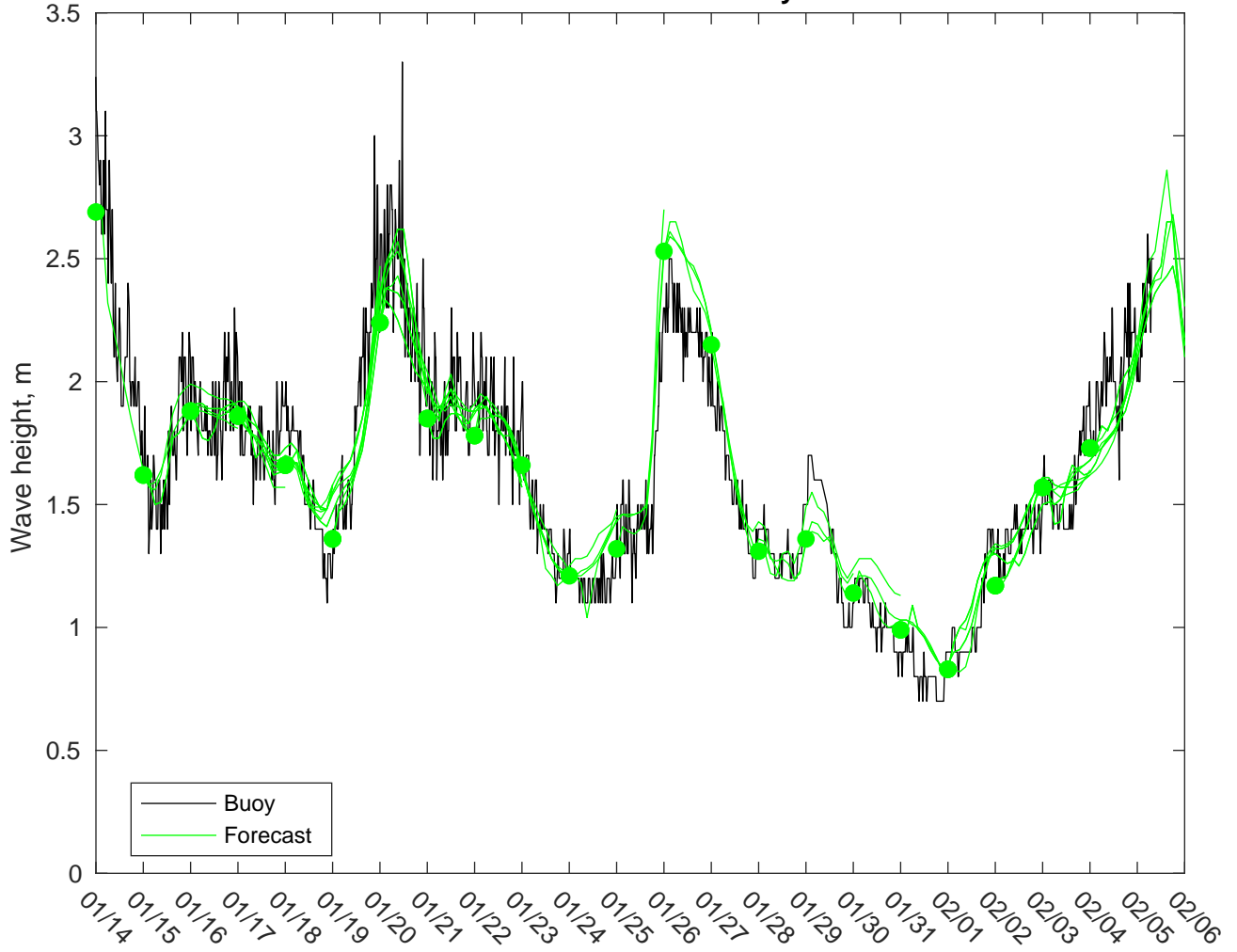
NDBC 46054 vs CMEMSWaves: 0 to 3 day forecast
