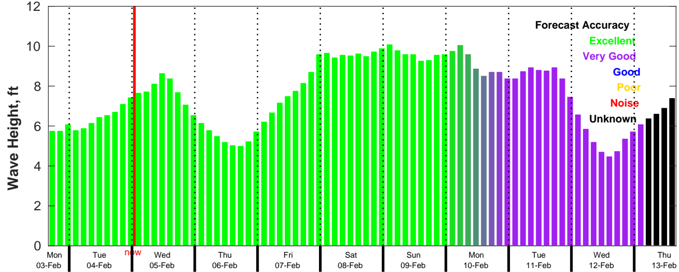
CMEMS Wave Forecast for NDBC 46069 from 03-Feb-2025 16:00:00 to 13-Feb-2025 16:00:00
