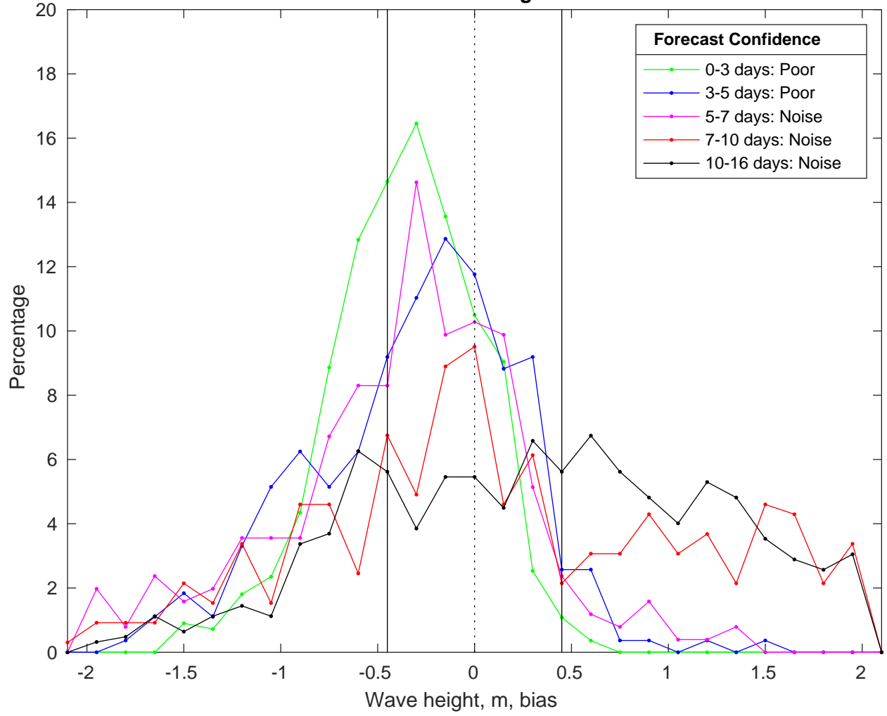
NDBC 46246 vs GFSWaves Bias Histogram: 05-Feb-2025
