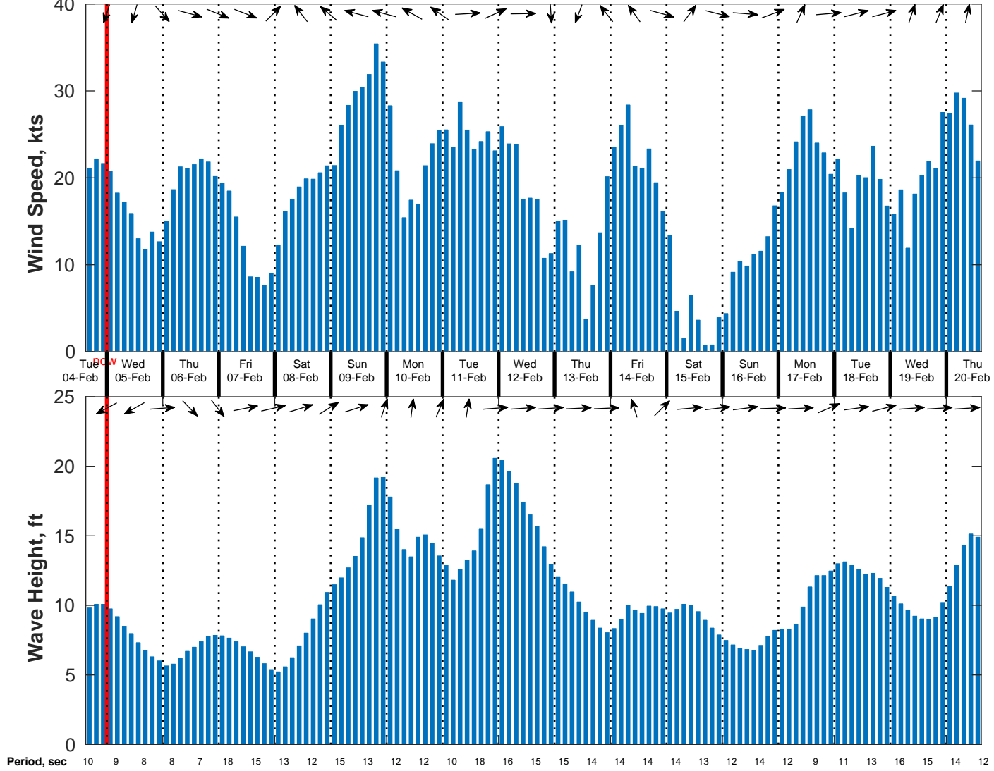
Wind & Wave Forecast for NDBC 46246 from 04-Feb-2025 15:00:00 to 20-Feb-2025 15:00:00
