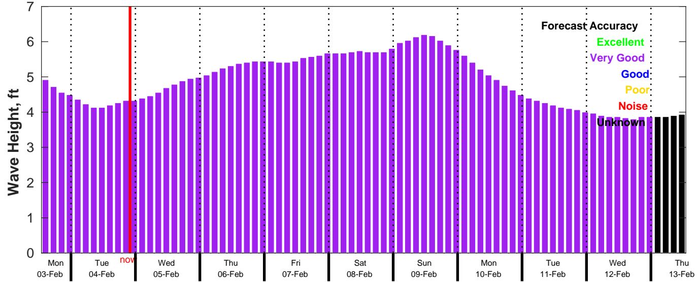
CMEMS Wave Forecast for NDBC 51209 from 03-Feb-2025 13:00:00 to 13-Feb-2025 13:00:00
