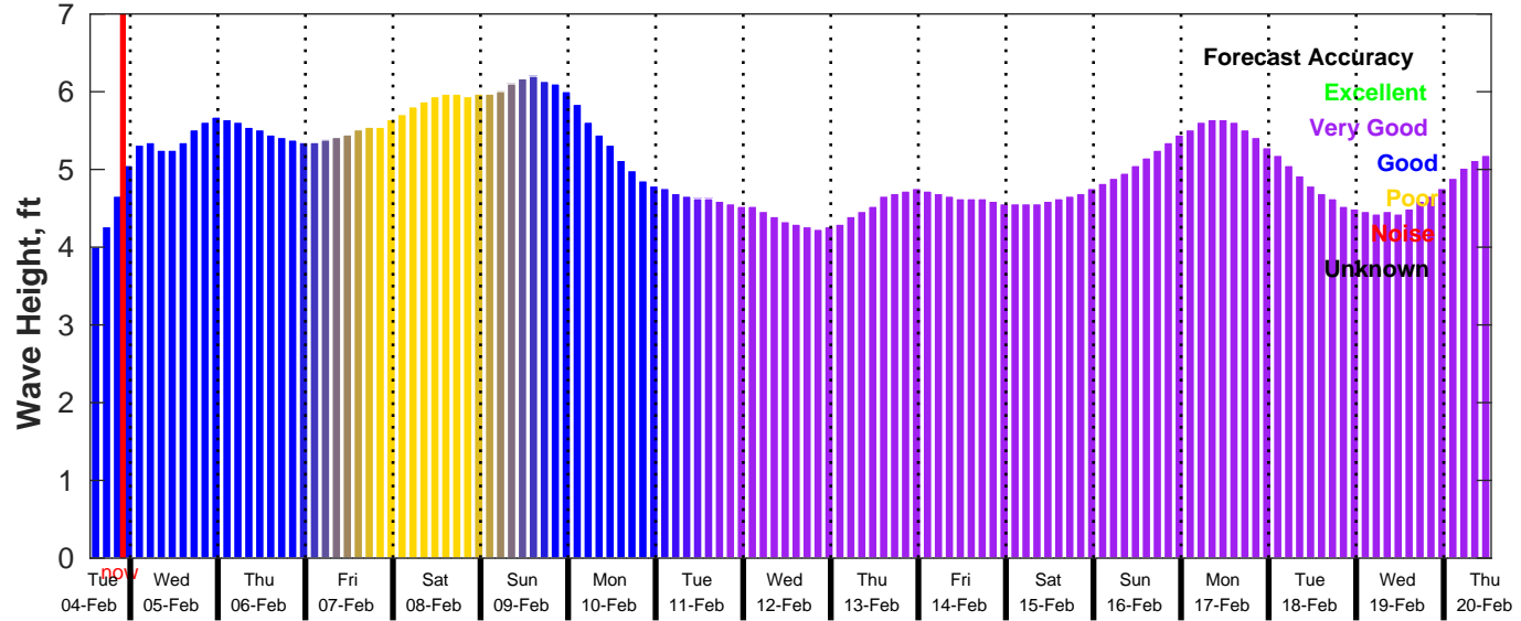
GFS Wave Forecast for NDBC 51209 from 04-Feb-2025 13:00:00 to 20-Feb-2025 13:00:00
