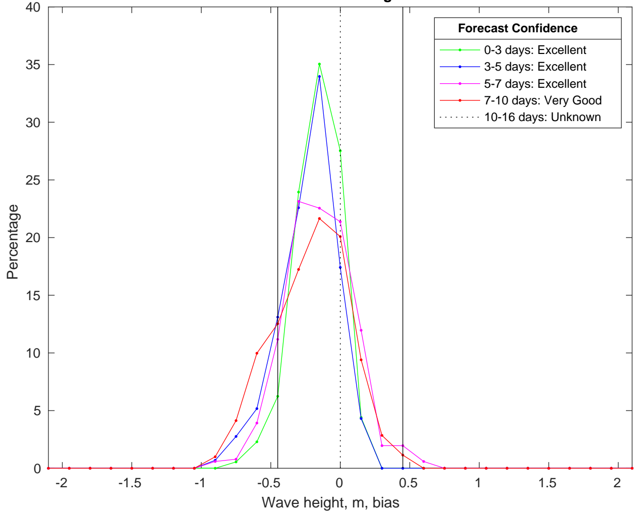
NDBC 52211 vs CMEMSWaves Bias Histogram: 05-Feb-2025
