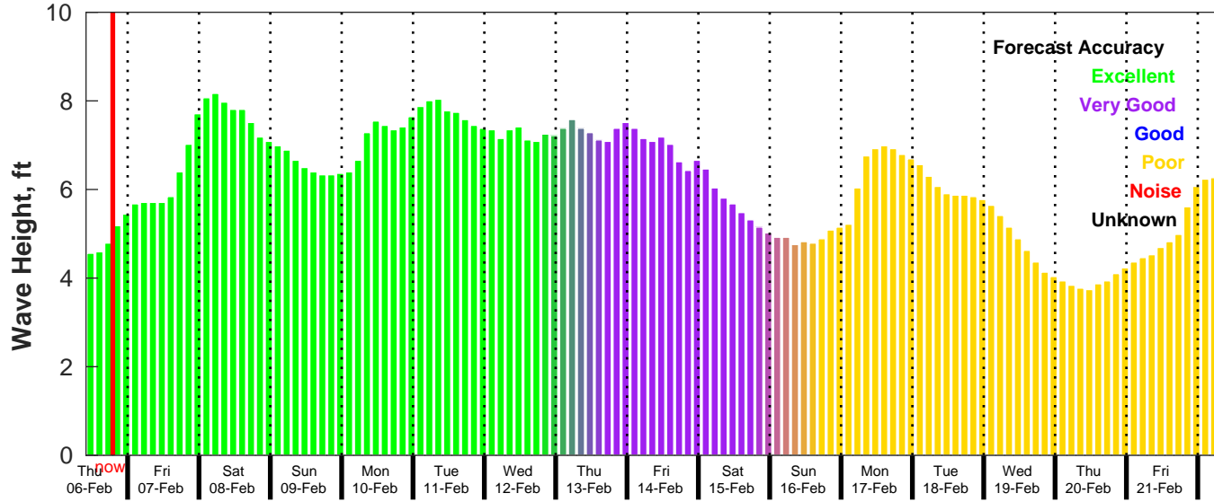
GFS Wave Forecast for NDBC 52211 from 05-Feb-2025 10:00:00 to 21-Feb-2025 10:00:00
