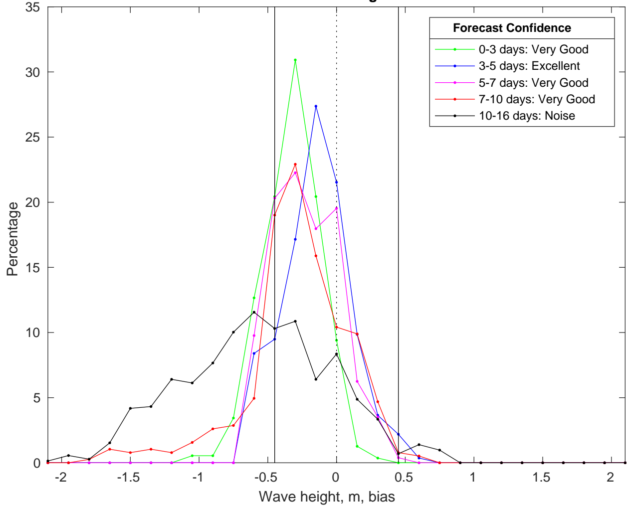
NDBC 52212 vs GFSWaves Bias Histogram: 05-Feb-2025
