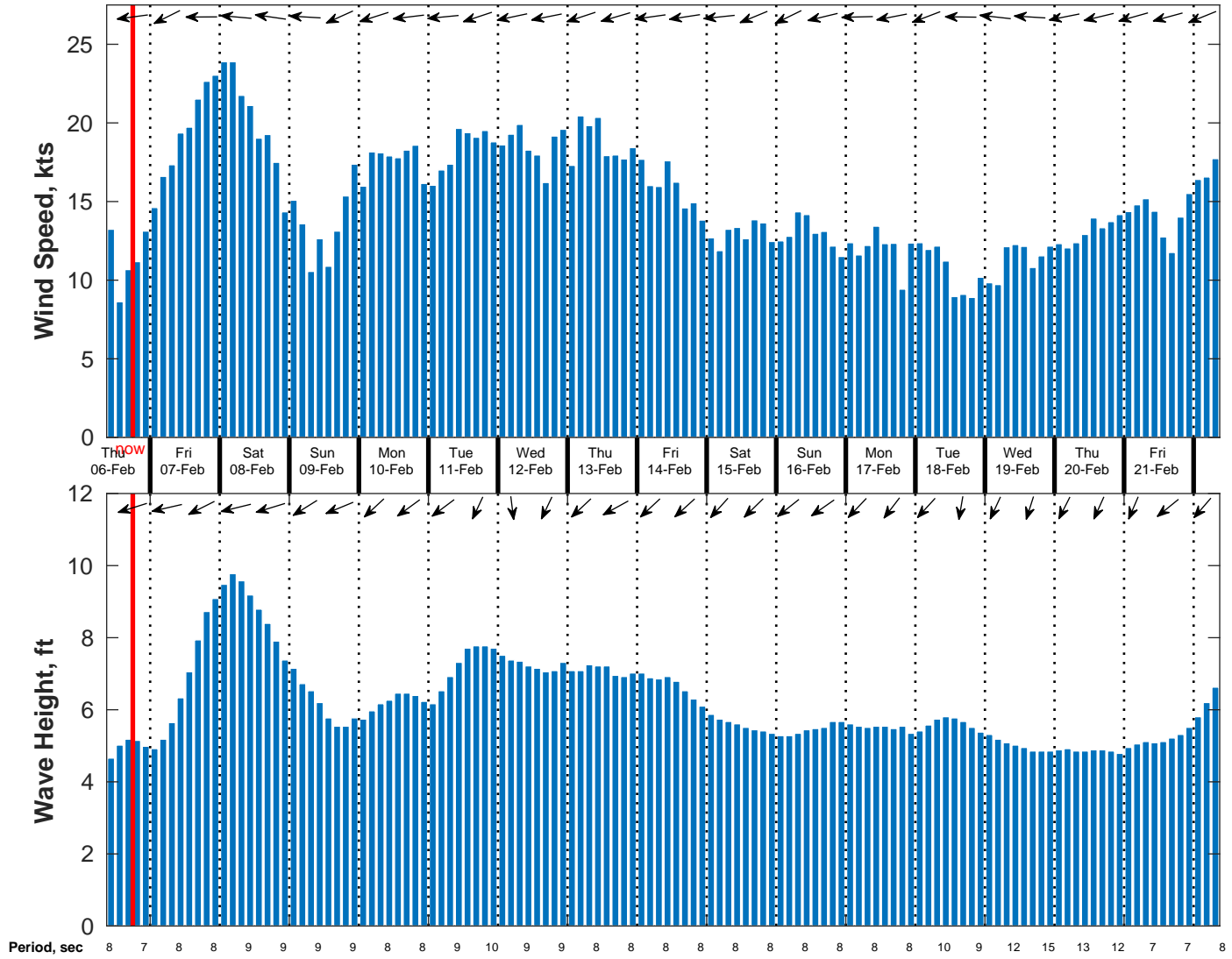
Wind & Wave Forecast for NDBC 52212 from 05-Feb-2025 09:00:00 to 21-Feb-2025 09:00:00
