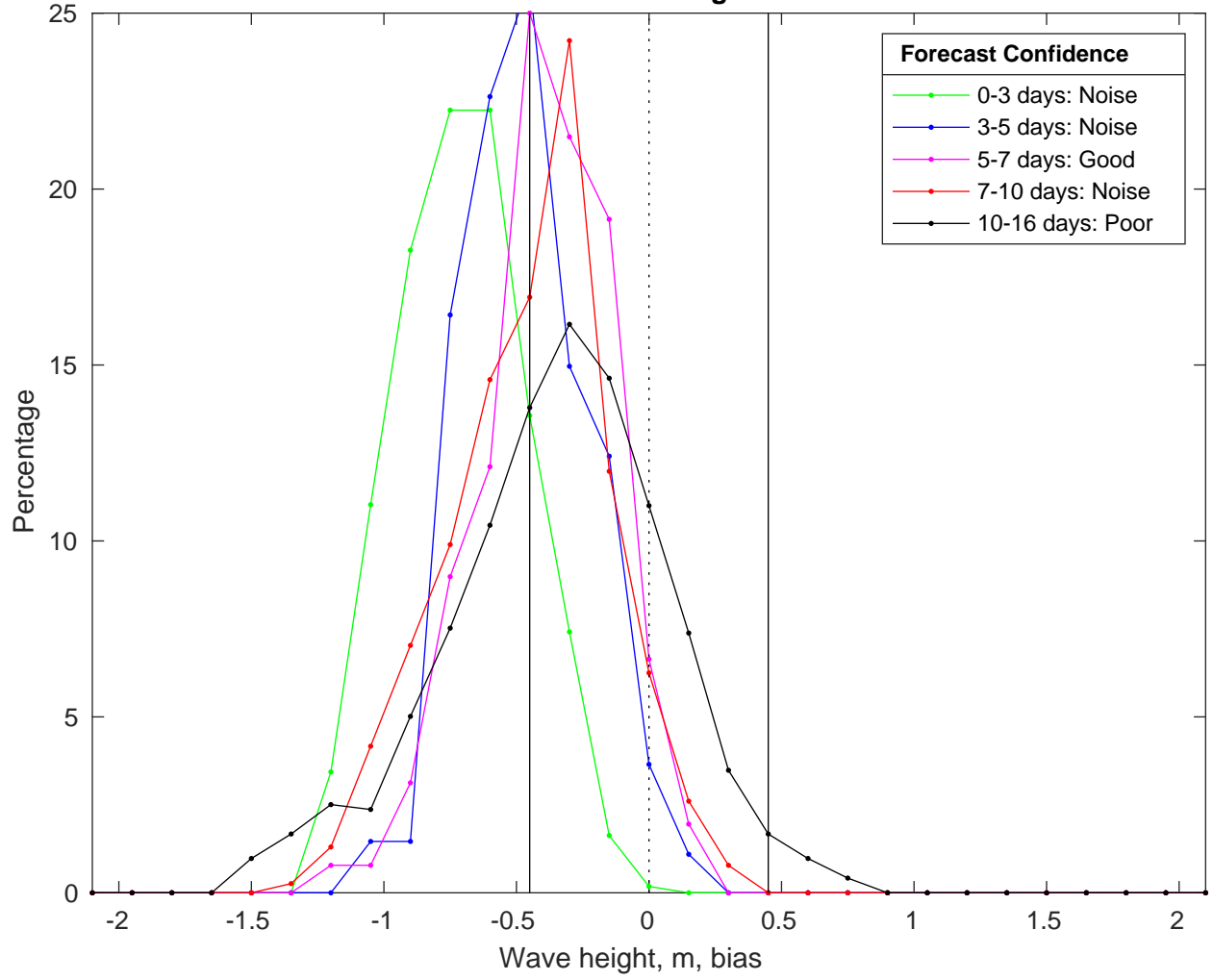
NDBC 52213 vs GFSWaves Bias Histogram: 05-Feb-2025
