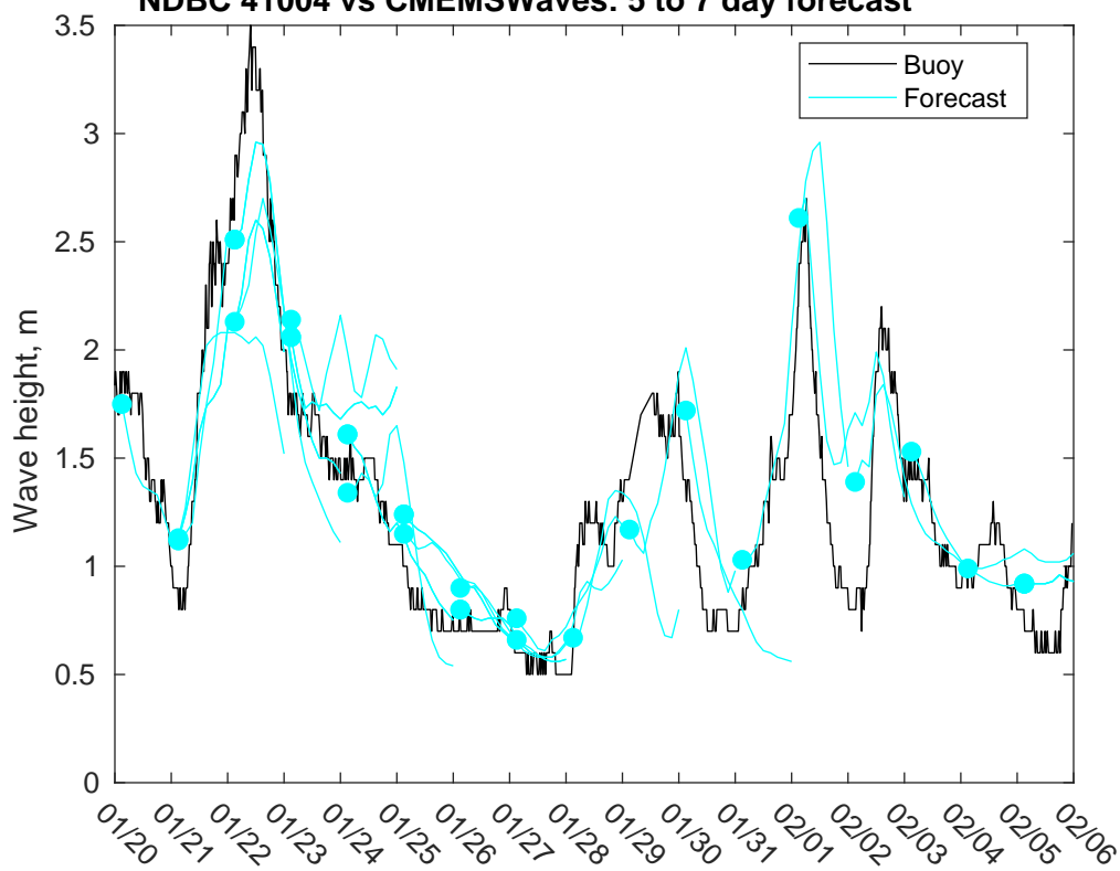
NDBC 41004 vs CMEMSWaves: 5 to 7 day forecast
