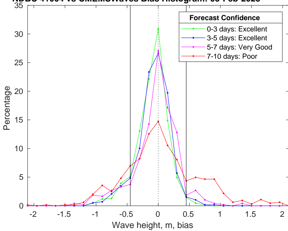
NDBC 41004 vs CMEMSWaves Bias Histogram: 05-Feb-2025
