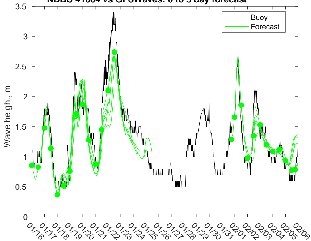
NDBC 41004 vs GFSWaves: 0 to 3 day forecast
