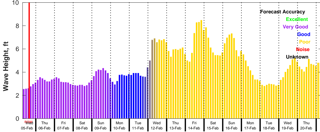
GFS Wave Forecast for NDBC 41004 from 05-Feb-2025 07:00:00 to 21-Feb-2025 07:00:00
