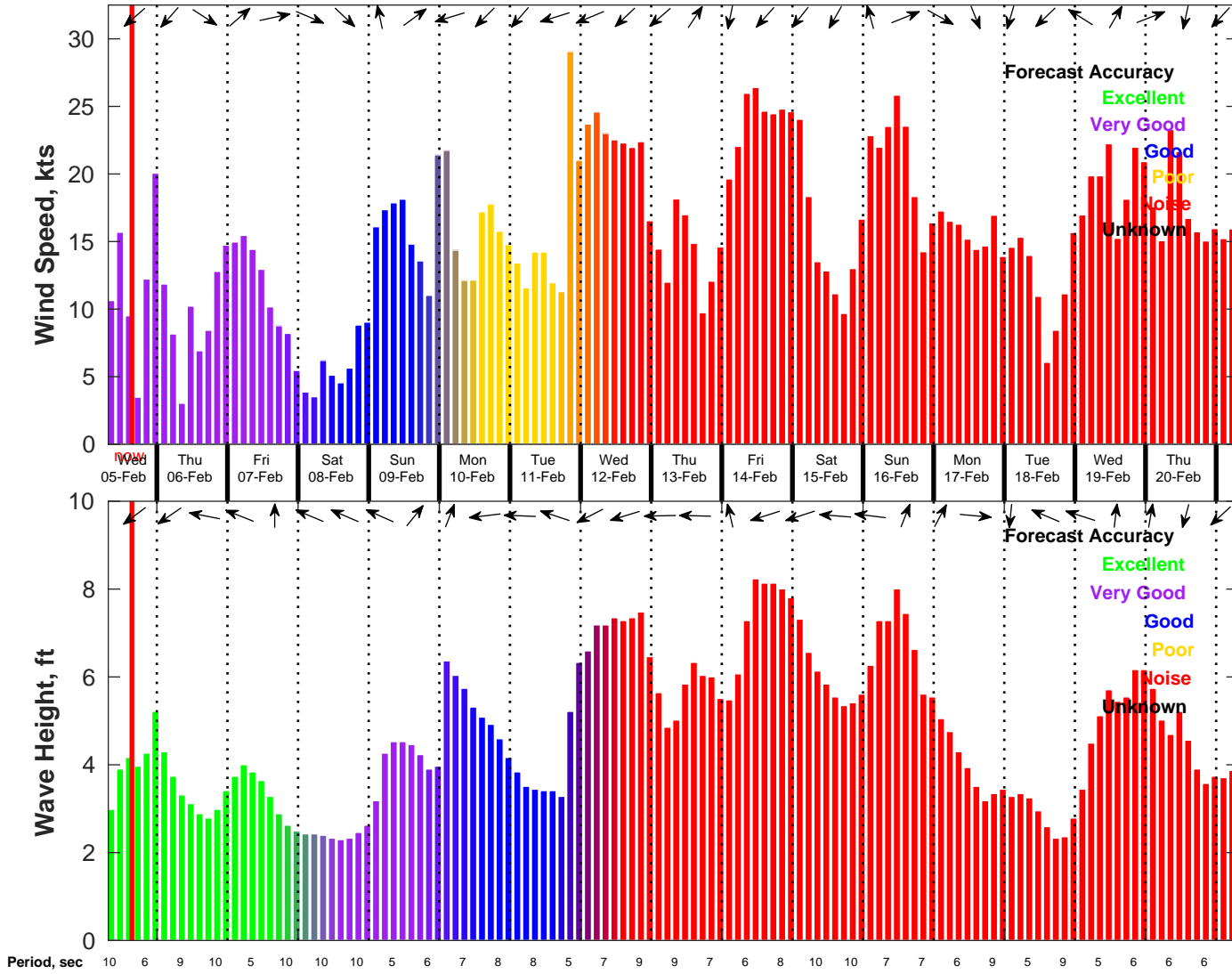
Wind & Wave Forecast for NDBC 41013 from 05-Feb-2025 07:00:00 to 21-Feb-2025 07:00:00
