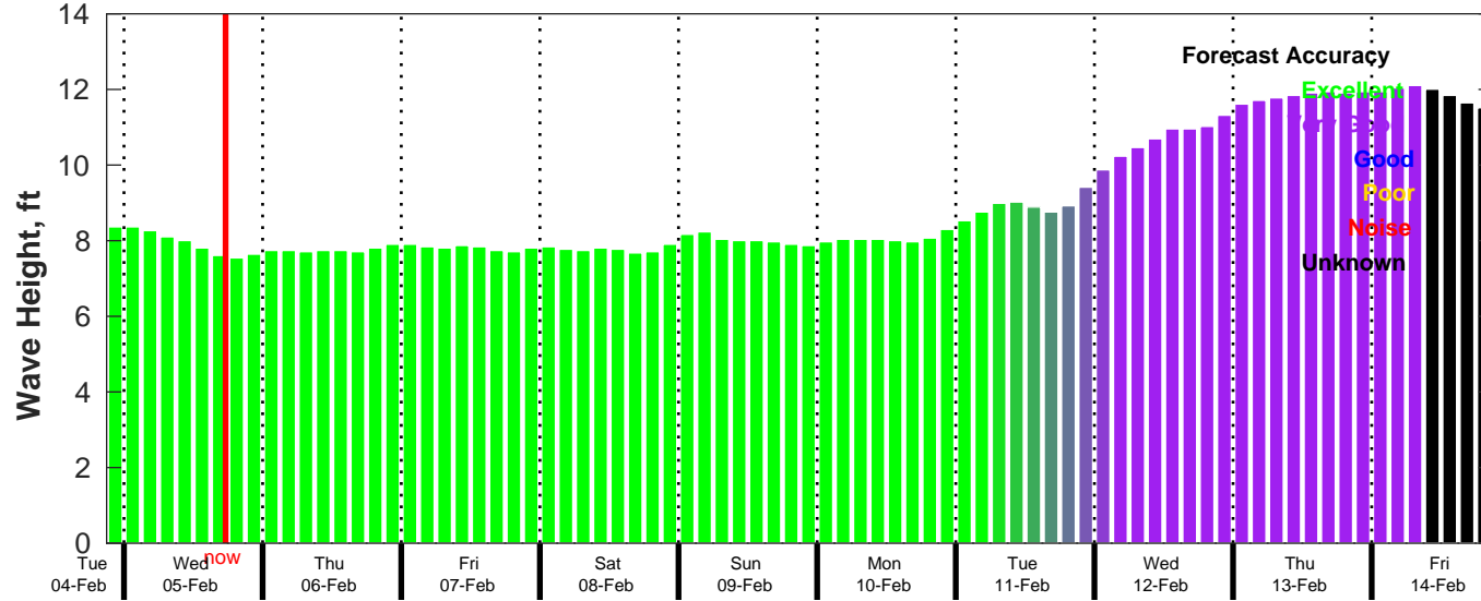
CMEMS Wave Forecast for NDBC 41040 from 04-Feb-2025 21:00:00 to 14-Feb-2025 21:00:00
