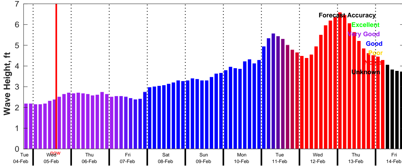
CMEMS Wave Forecast for NDBC 42020 from 04-Feb-2025 18:00:00 to 14-Feb-2025 18:00:00
