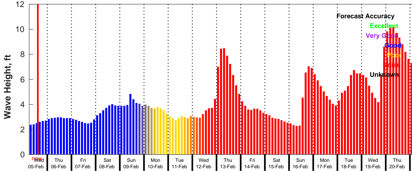
GFS Wave Forecast for NDBC 42020 from 05-Feb-2025 06:00:00 to 21-Feb-2025 06:00:00
