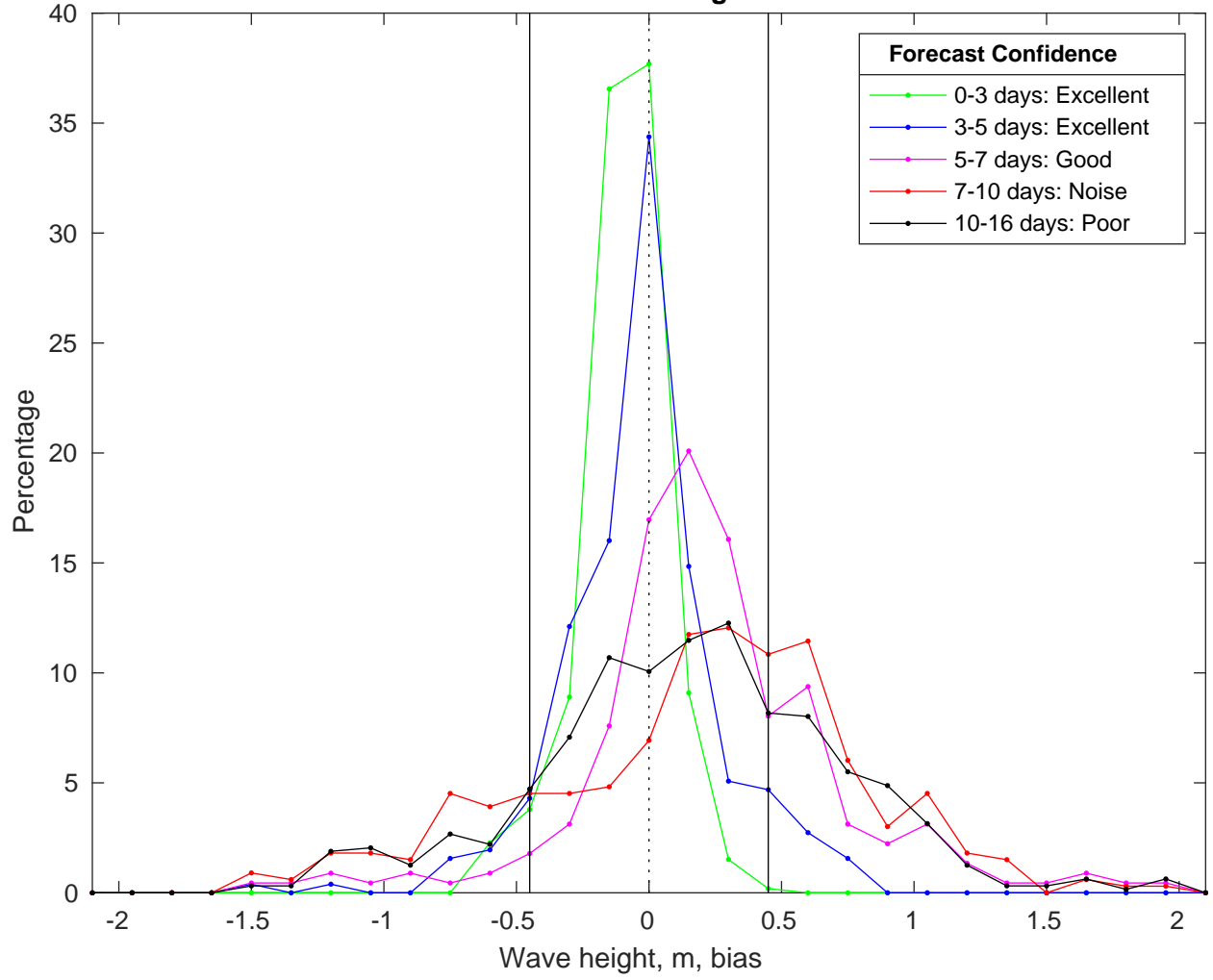
NDBC 42035 vs GFSWaves Bias Histogram: 05-Feb-2025
