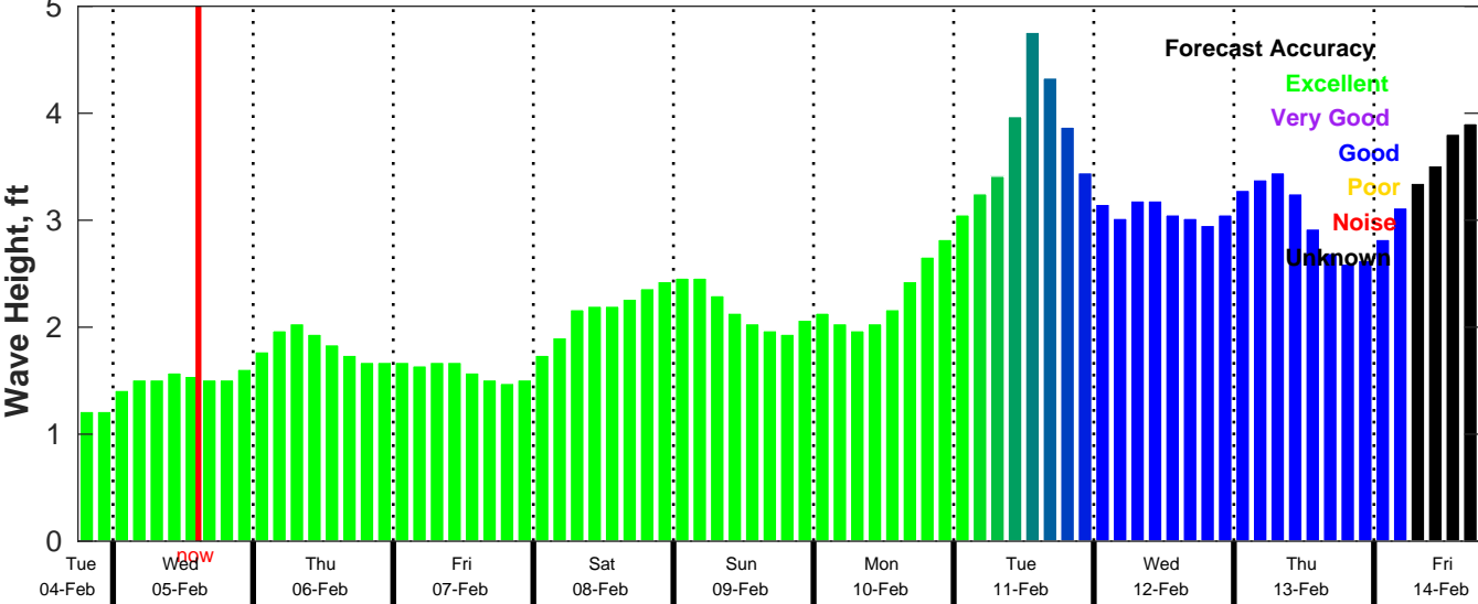
CMEMS Wave Forecast for NDBC 42035 from 04-Feb-2025 18:00:00 to 14-Feb-2025 18:00:00
