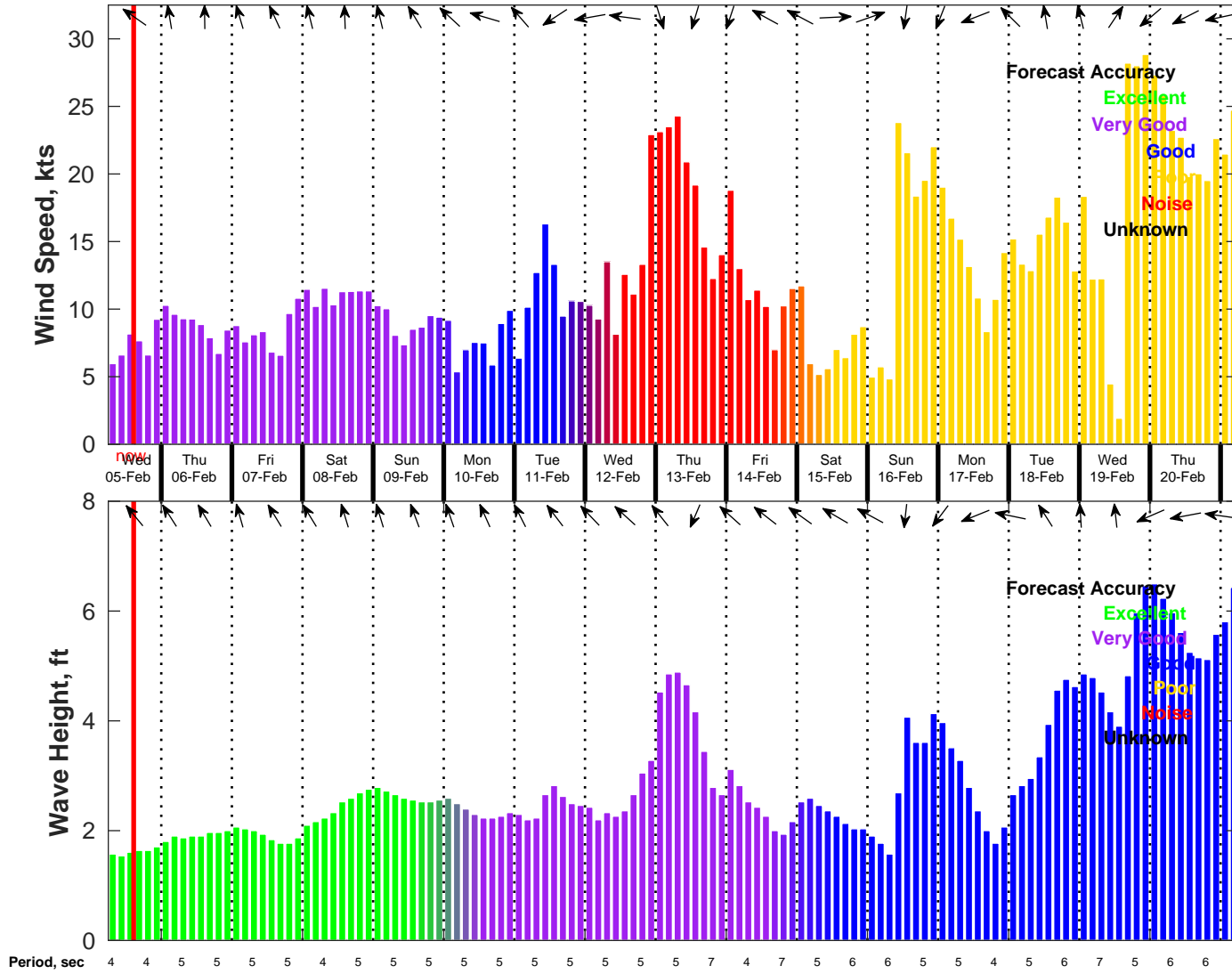
Wind & Wave Forecast for NDBC 42035 from 05-Feb-2025 06:00:00 to 21-Feb-2025 06:00:00
