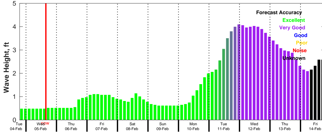
CMEMS Wave Forecast for NDBC 42036 from 04-Feb-2025 19:00:00 to 14-Feb-2025 19:00:00
