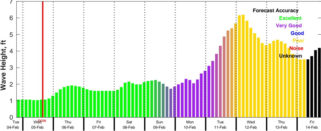
CMEMS Wave Forecast for NDBC 42040 from 04-Feb-2025 19:00:00 to 14-Feb-2025 19:00:00
