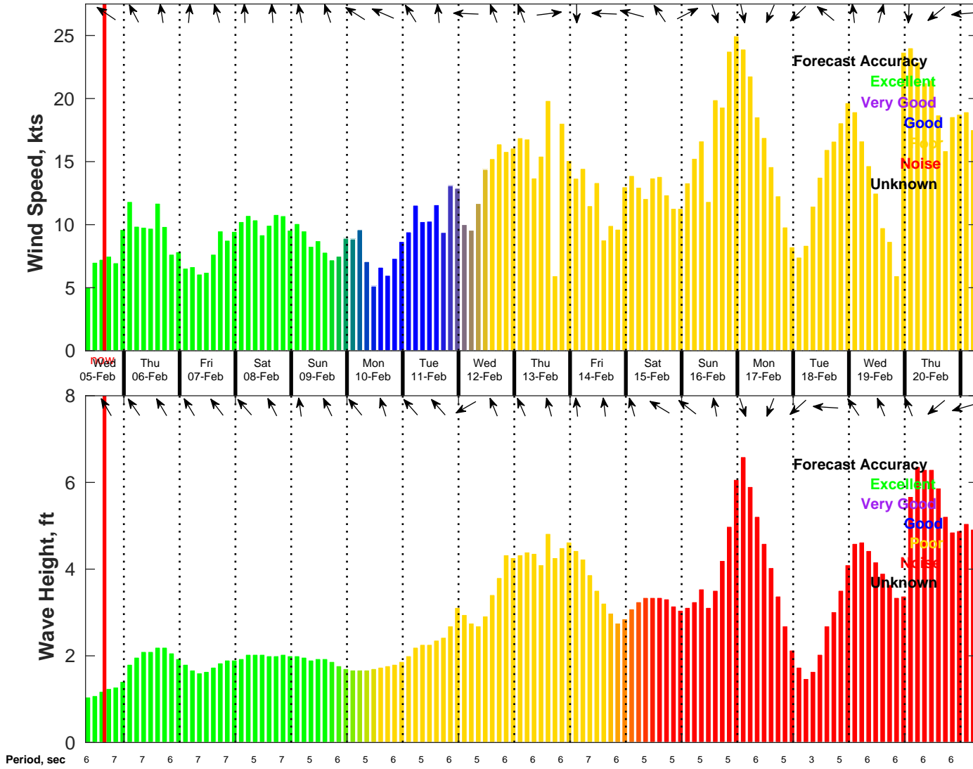
Wind & Wave Forecast for NDBC 42040 from 05-Feb-2025 07:00:00 to 21-Feb-2025 07:00:00
