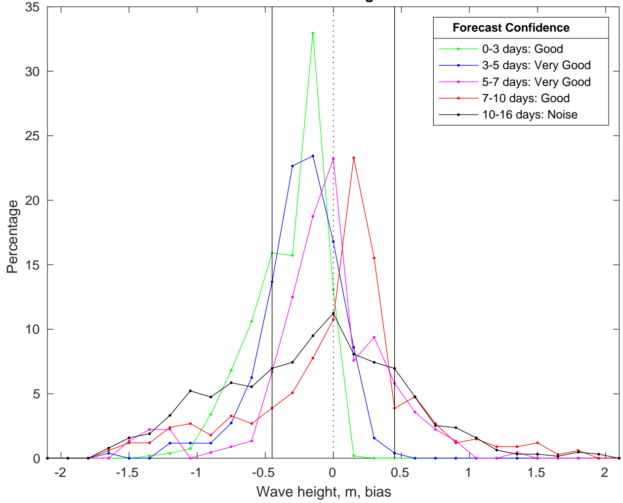
NDBC 42084 vs GFSWaves Bias Histogram: 05-Feb-2025
