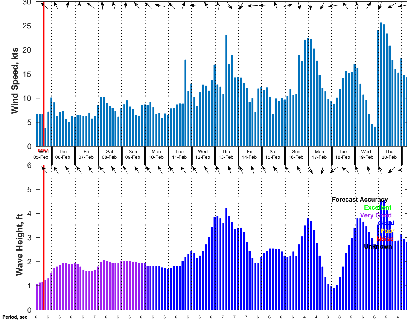
Wind & Wave Forecast for NDBC 42084 from 05-Feb-2025 07:00:00 to 21-Feb-2025 07:00:00
