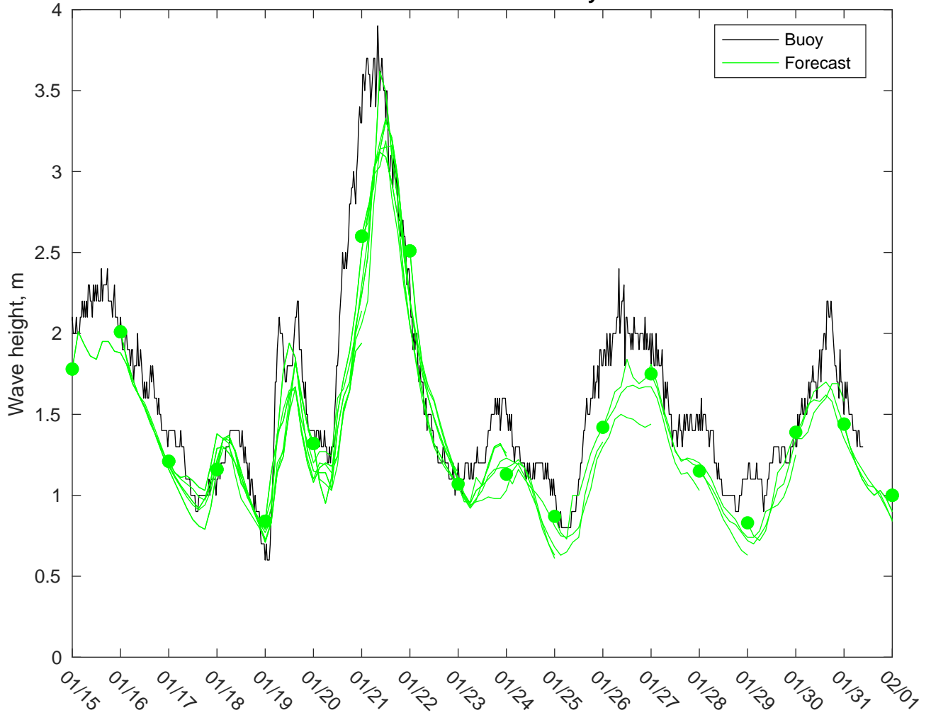
NDBC 42092 vs CMEMSWaves: 0 to 3 day forecast
