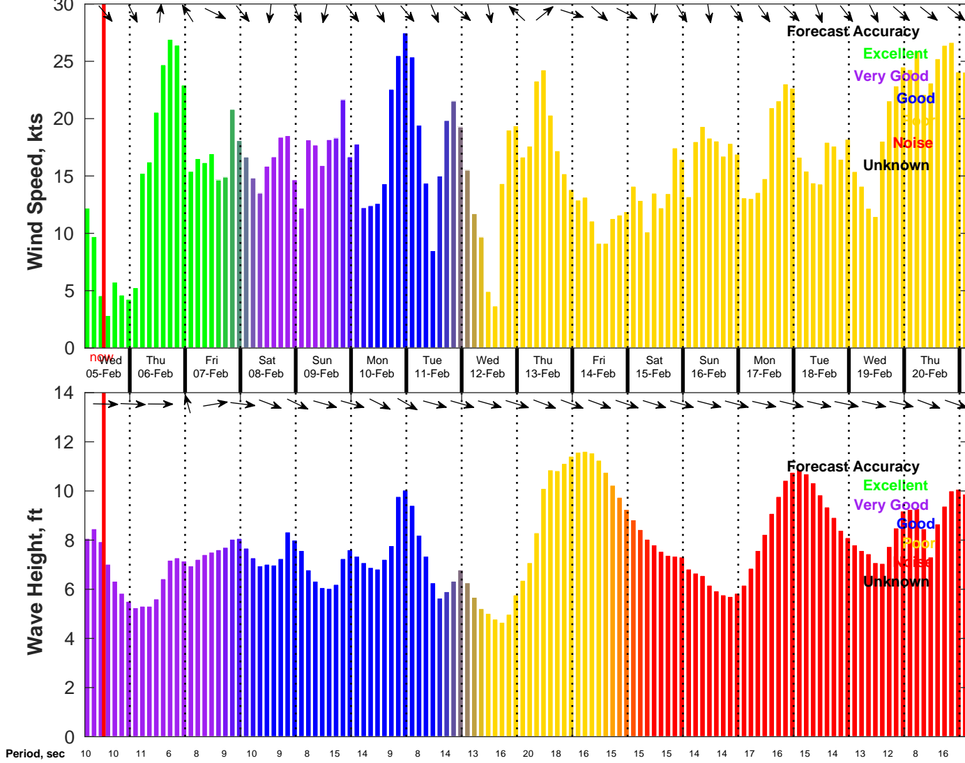
Wind & Wave Forecast for NDBC 46011 from 05-Feb-2025 04:00:00 to 21-Feb-2025 04:00:00
